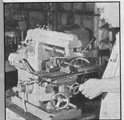
STEP MILLING
