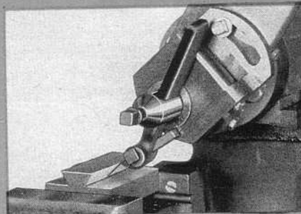
DOVETAILING
