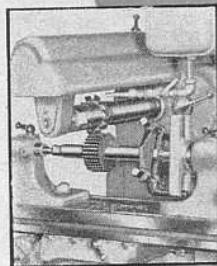
GEAR CUTTING
