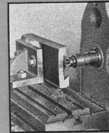
DOVETAILING
