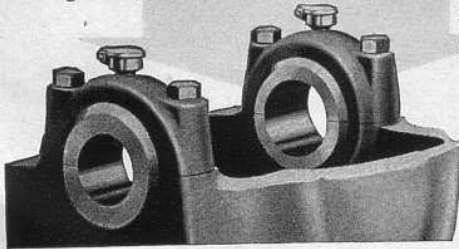
Custom-Bored High-Speed Babbitt HEADSTOCK SPINDLE BEARINGS
