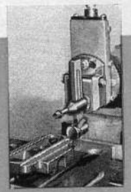
HORIZONTAL CUTS (Work Bolted to Table Top)
