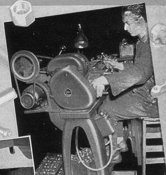
Machining forged terminals for aircraft, a continuous close-tolerance facing operation on economical basis.
