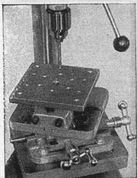
Typical spacing job for the W68 vise — drilling holes at 60^\circ intervals around center of drill jig.
