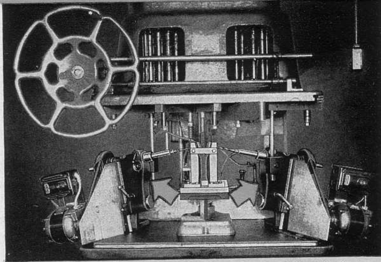
Two 63-series Atlas drilling heads teamed up with multiple spindle drill. Bracket being drilled requires five holes, two of them at an angle to both vertical and horizontal planes. Universal angle bracket holds each head in position — rams attached to multiple spindle head automatically actuate the angular feeds. Drilling time has been reduced by more than 60 per cent — and the cost of a special drilling machine is eliminated.
