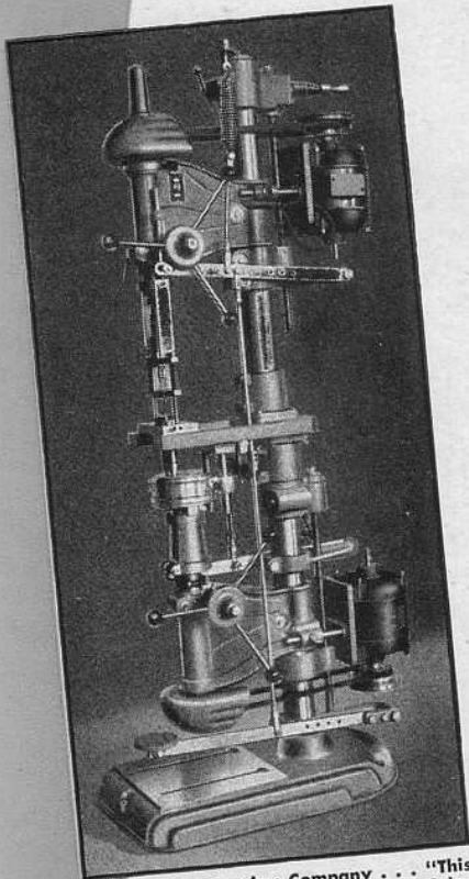
The Bastion-Blessing Company . . . "This drilling machine, built around two Atlas drill press heads and standard column and base, increased production to over 4,000 holes drilled per hour."
