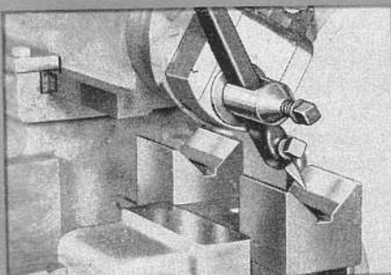
V-CUTS
