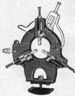
STEADY REST
