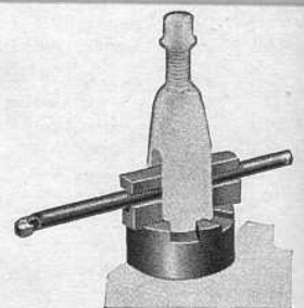
BORING TOOL HOLDER
