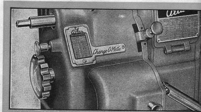
Close-up view of MFB Atlas milling machine showing Change-O-Matic controls. Notice (1) large notched knob and index plunger for selecting feed; (2) chart window showing feed selected; (3) tumbler lever controlling direction of table travel; (4) feed gear case; and (5) portion of telescoping drive bar to the table feed screw.
