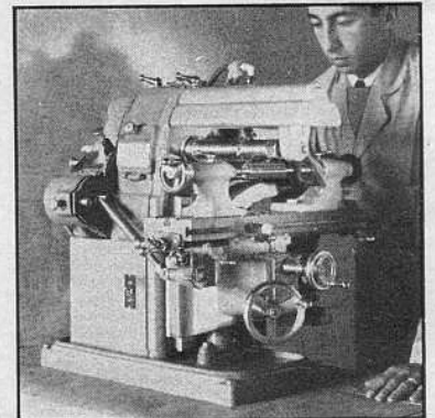
SPLINING
